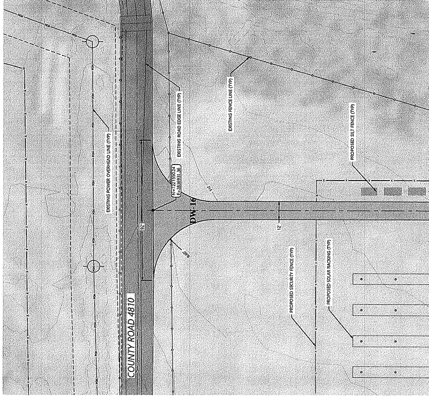
DW-16 COUNTY ROAD 4810 ENTRANCES 02
