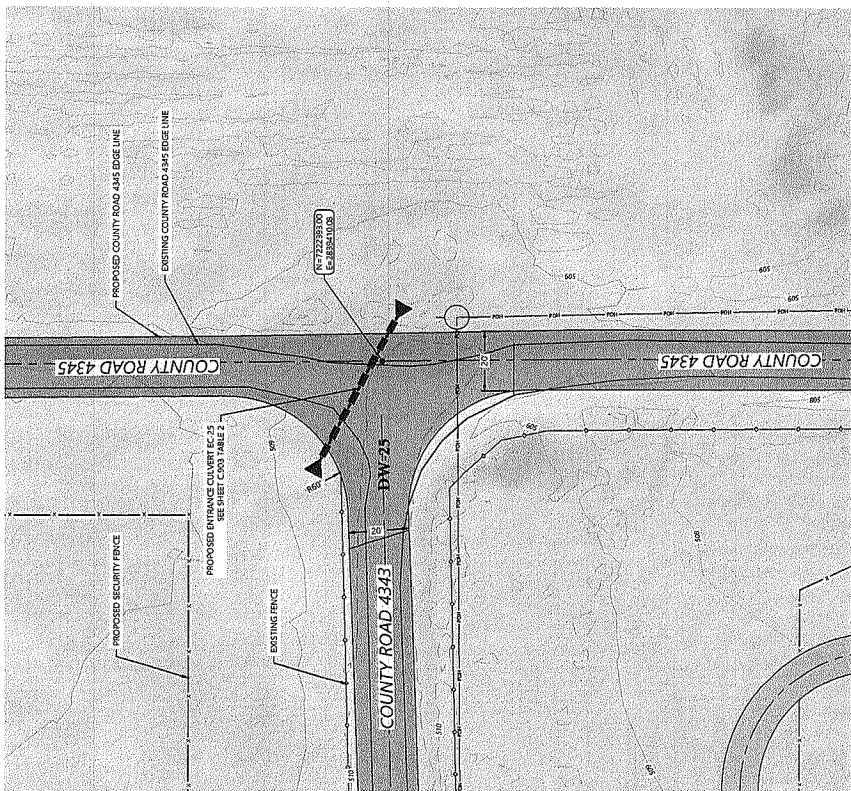
DW-25 COUNTY ROAD 4343 - COUNTY ROAD 4345 ENTRANCE 01
