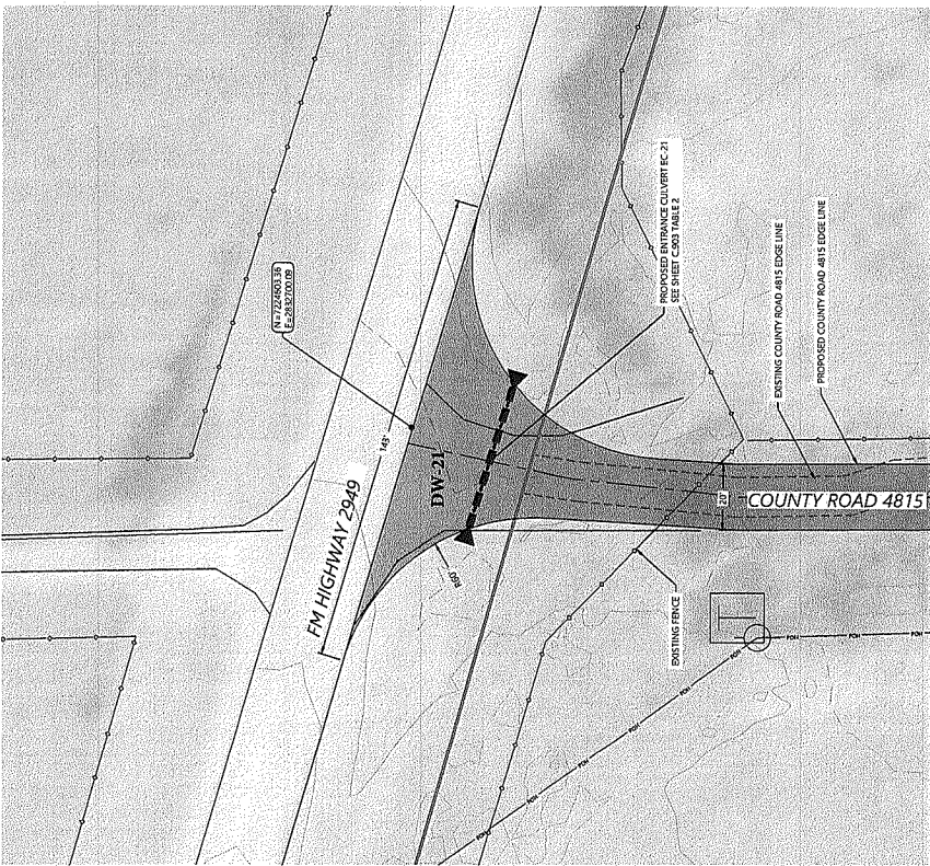
DW-21 COUNTY ROAD 4815 - FM 2929 ENTRANCE 01
