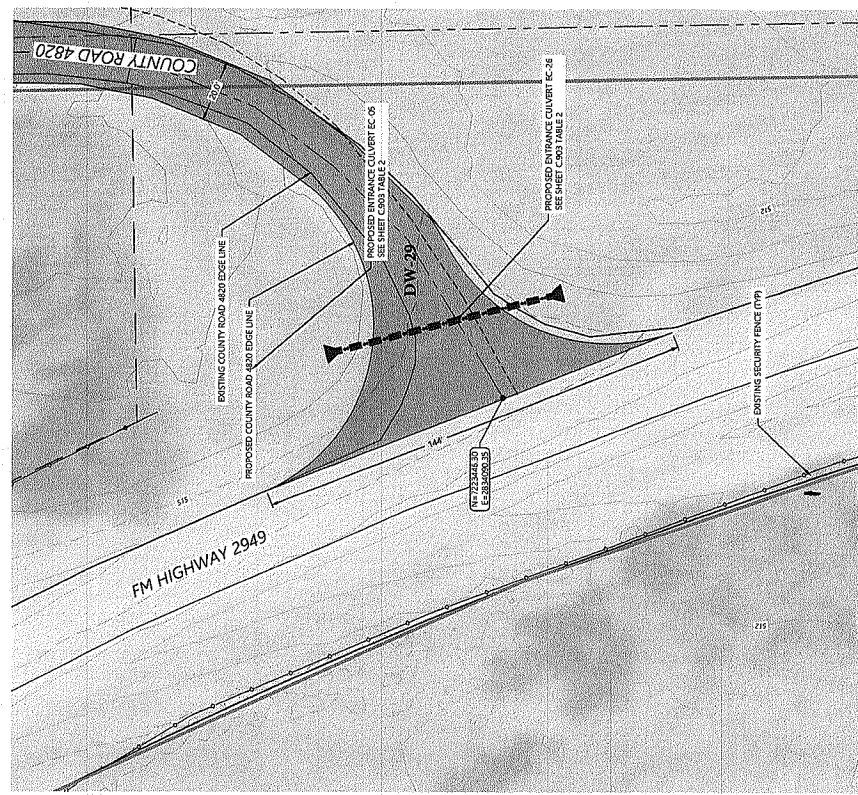
DW-29 COUNTY ROAD 4820 - FM 2949 ENTRANCES 01 (out of sequence number)
