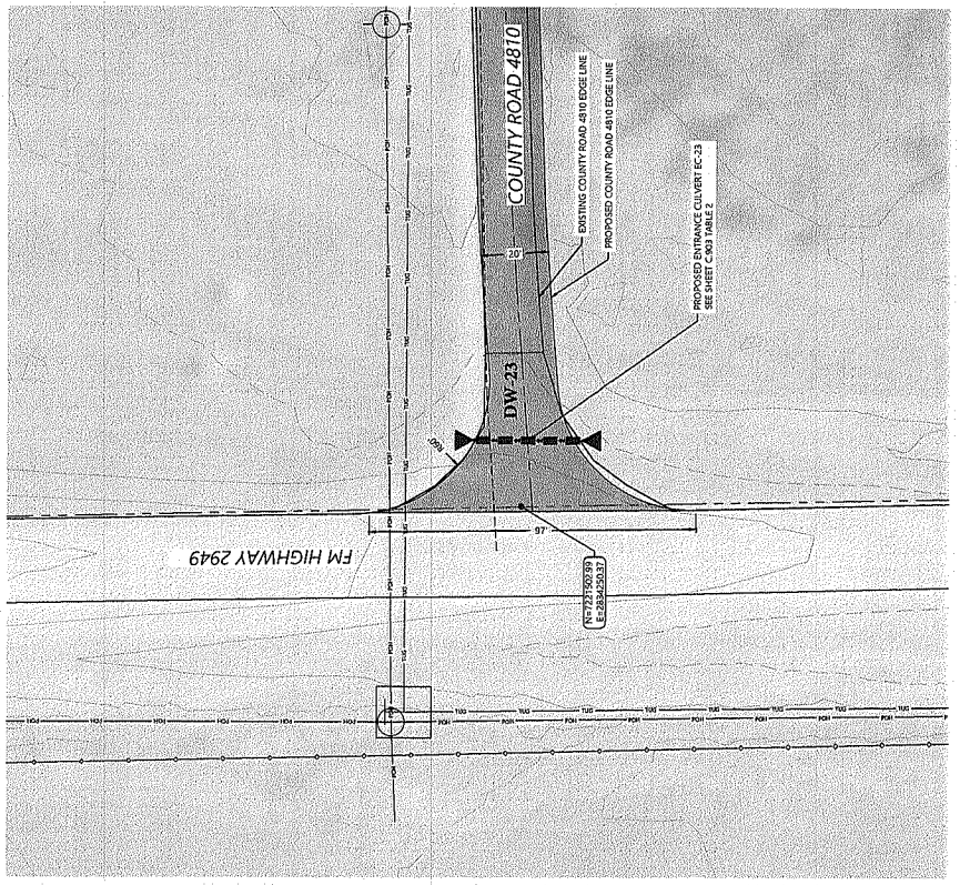
DW-23 COUNTY ROAD 4810 - FM 2949 ENTRANCE 01
