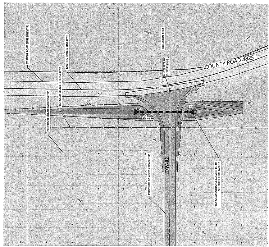
DW-02 COUNTY ROAD 4825 ENTRANCES 02
