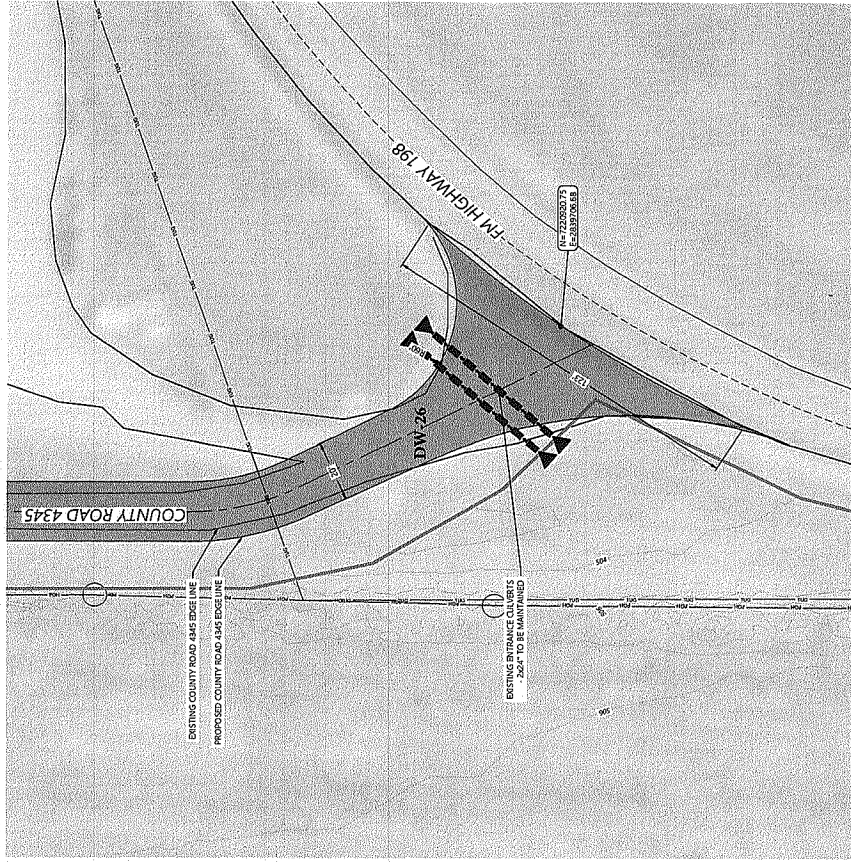
DW-26 COUNTY ROAD 4345 - FM 198 ENTRANCE 01
